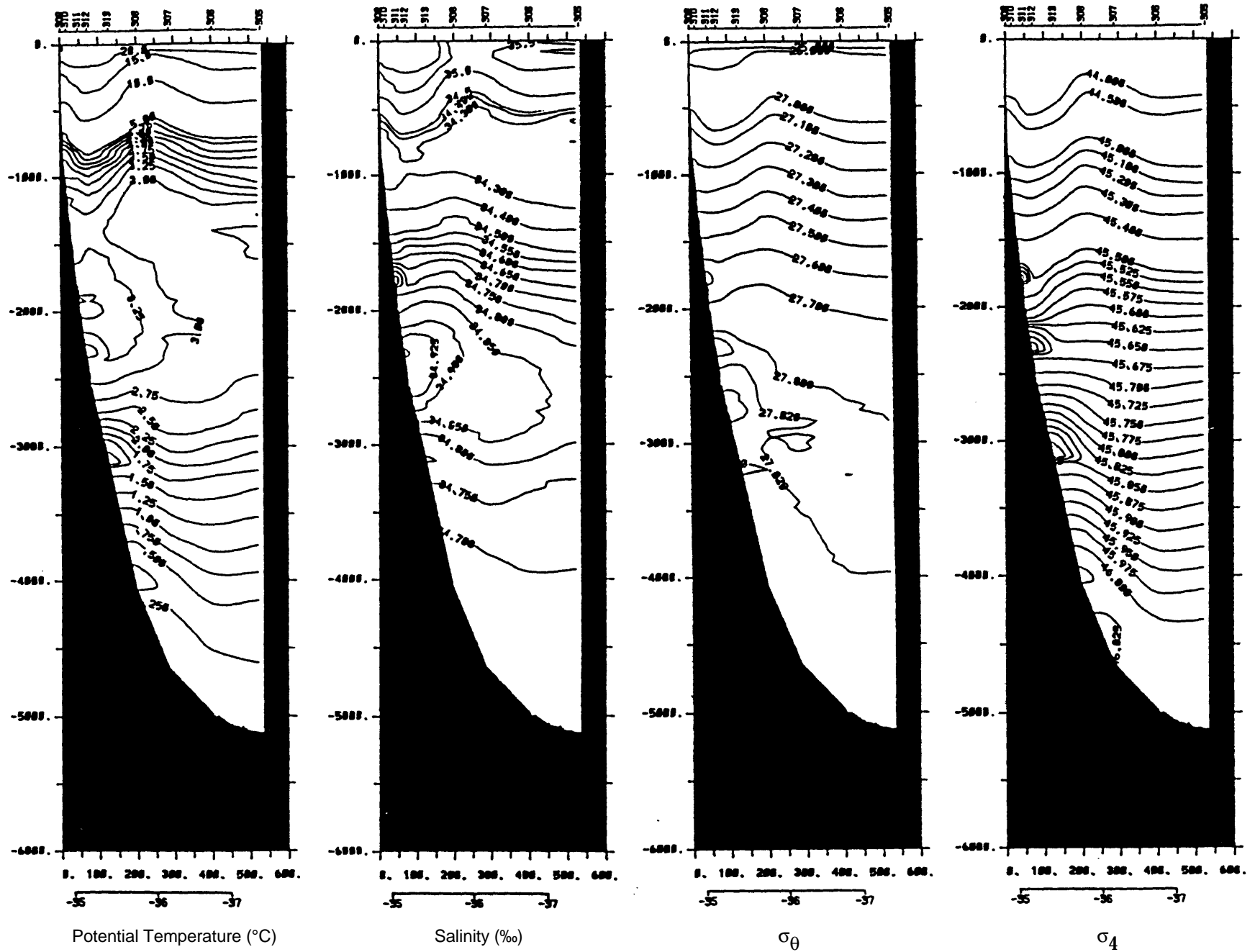
Vertical sections of CTD data from Brazil Current portion of Hydros 3 and 4 (Potential Temperature, Salinity, \sigma_{\theta} and \sigma_4 ). The objective mapping routine causes the fallacious extrema at the boundary.
